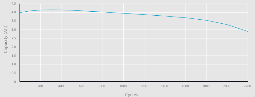
Charge at C/3 - discharge at 2 A
